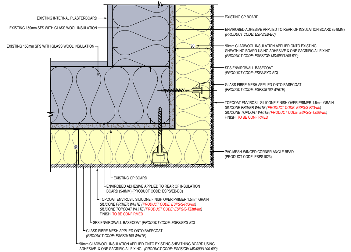
02 PLAN SECTION - RENDER EXTERNAL CORNER DETAIL (SFS) Scale 1:3
