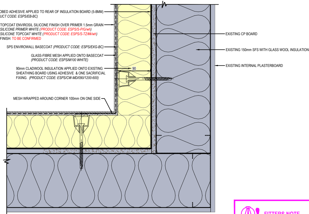
03 PLAN SECTION - RENDER INTERNAL CORNER DETAIL (SFS) Scale 1:3
