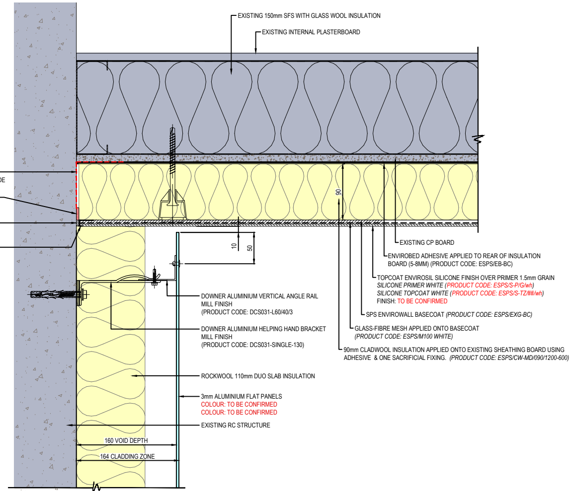
04 PLAN SECTION - RENDER / ALUMINIUM PANEL INTERNAL CORNER DETAIL Scale 1:3
